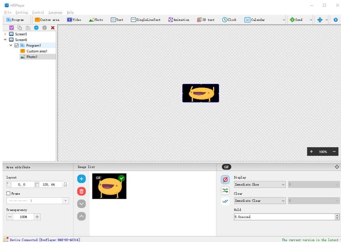
Figure 4-12 Gif attributes
