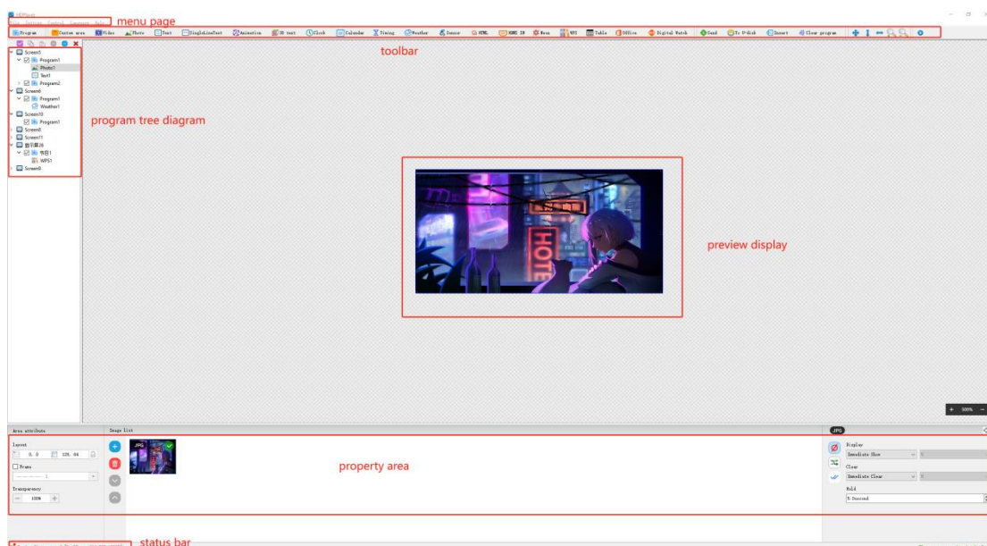
Figure 4-1 Software interface
