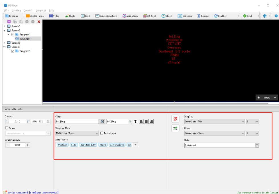
Figure 4- 44 Weather attributes
