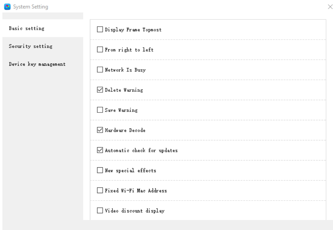
Figure 6-1 System settings
