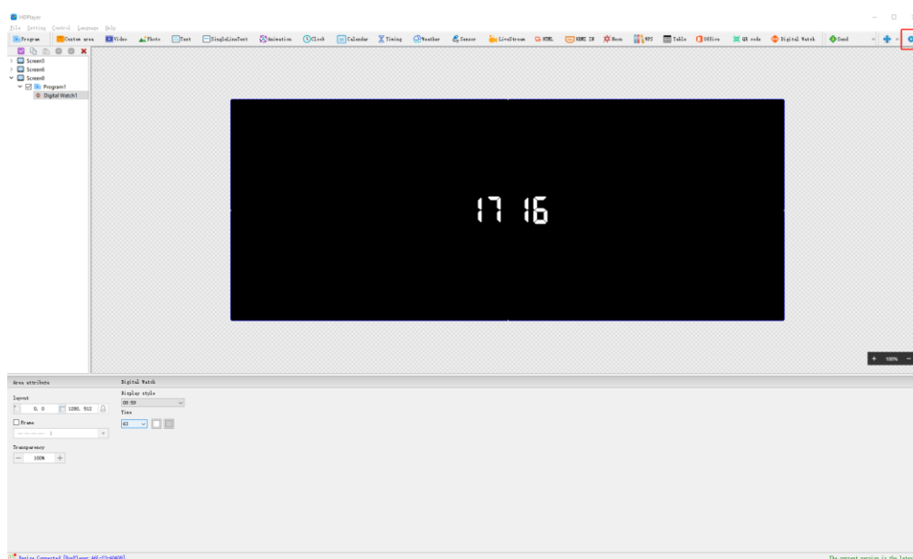
Figure 4-3 9 program preview
