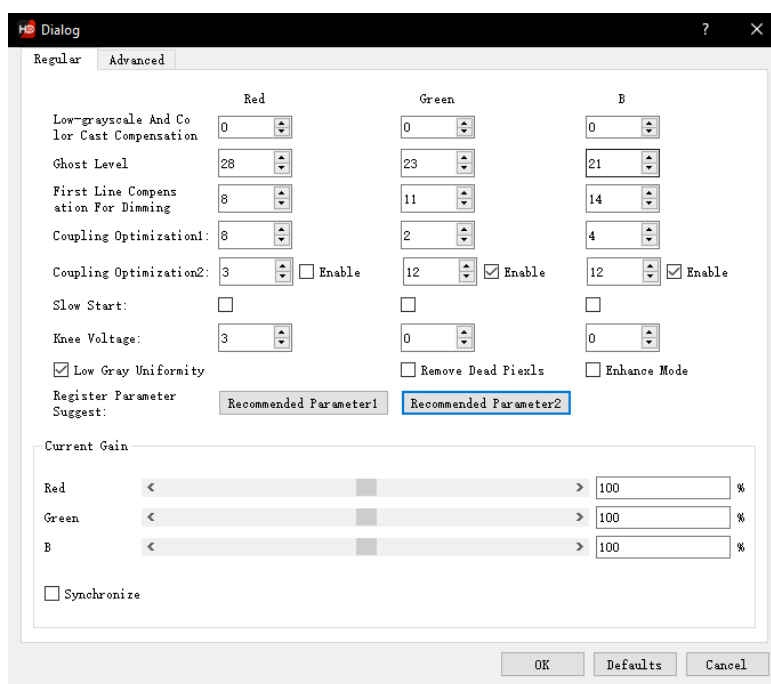
Figure 3-8 Extended attributes
