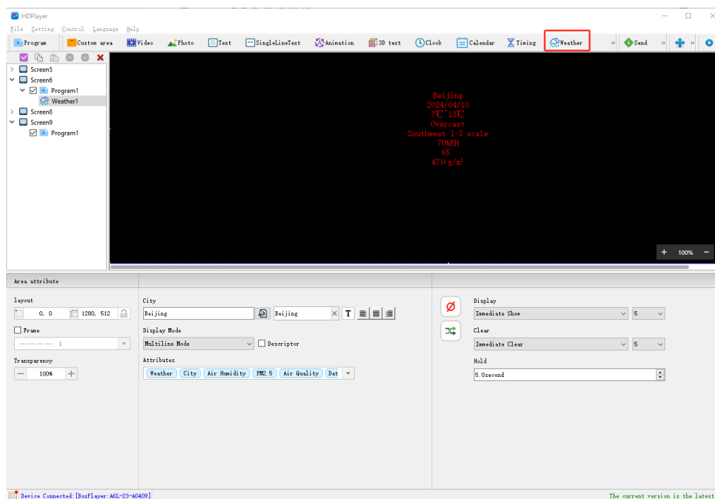
Figure 4- 43 Add "Weather"
