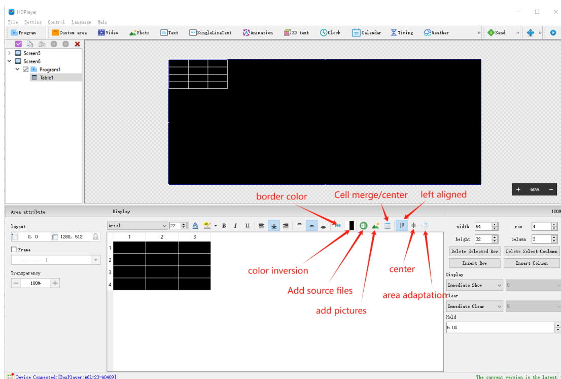
Figure 4-1 5 WPS properties
