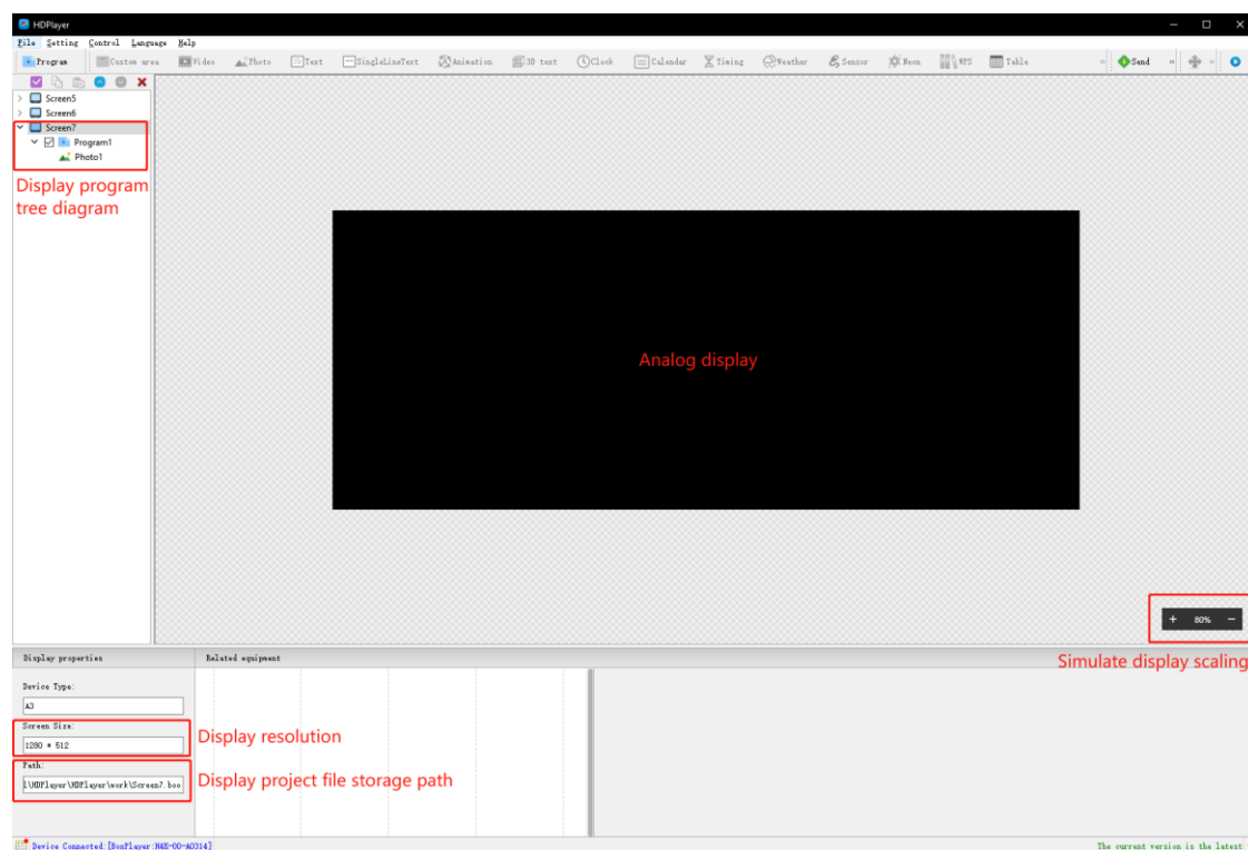
Figure 4-4 Display properties
