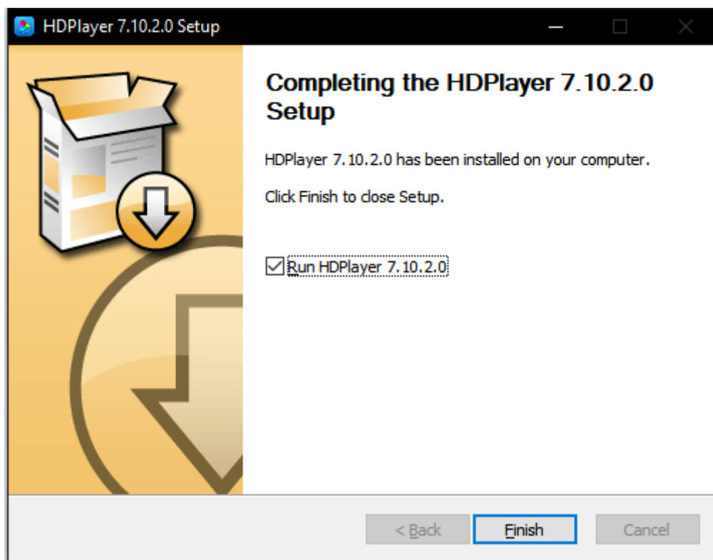
Figure 1-2 Installation Wizard
