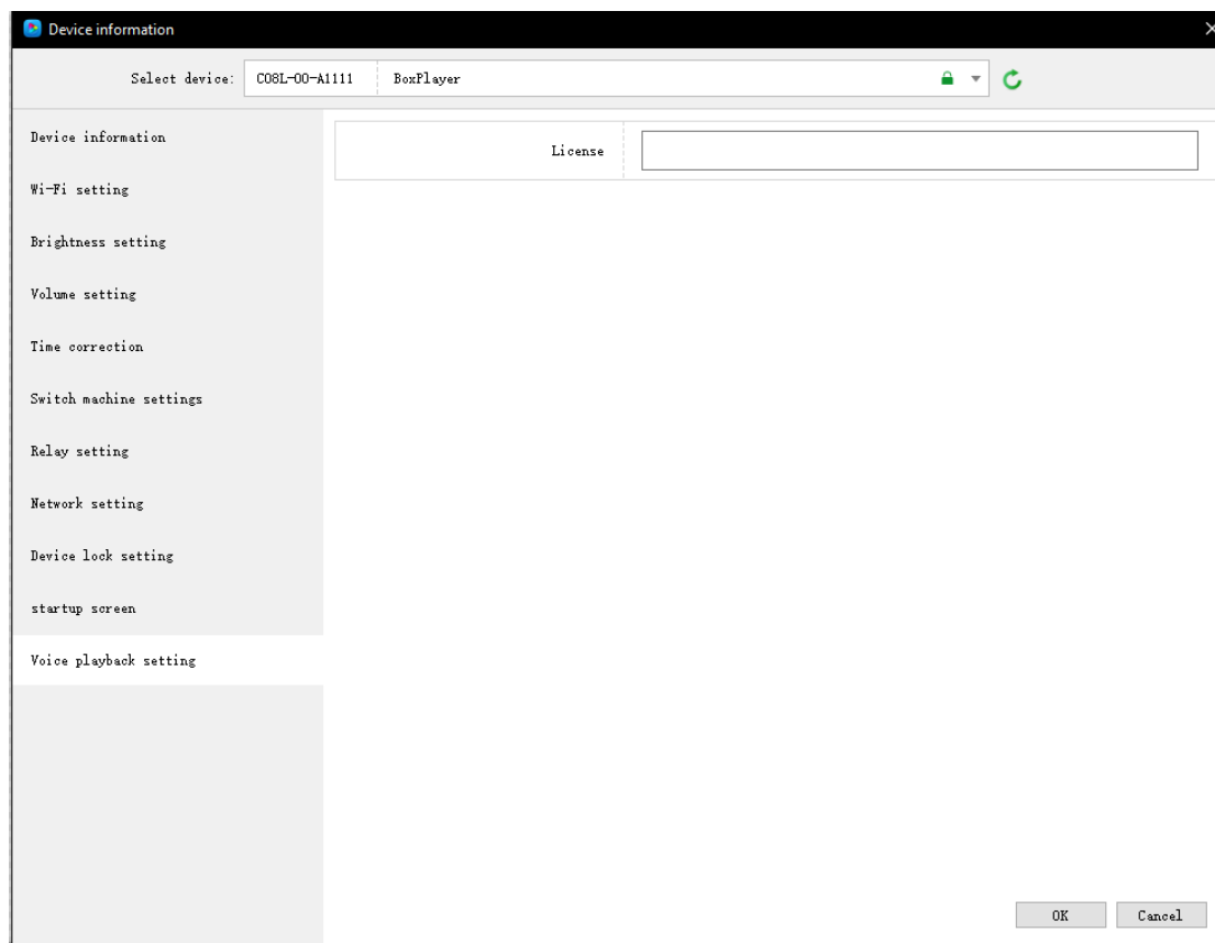
Figure 1-1 Inactive page
