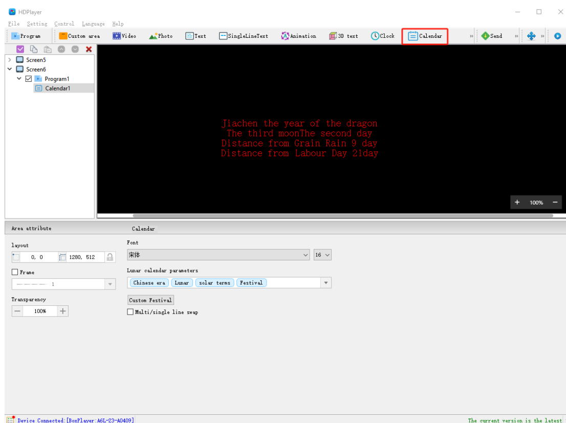
Figure 4-2 8 Add timing
