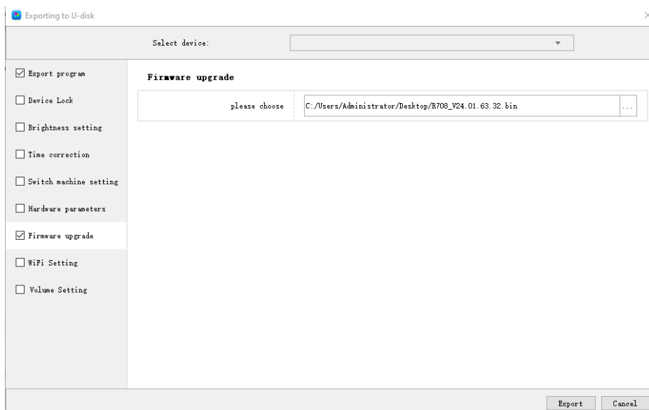
Figure 5-10 Firmware upgrade
