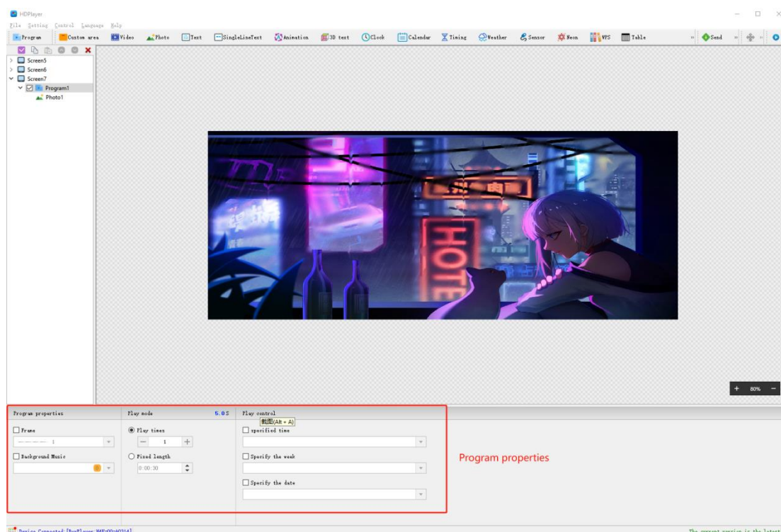
Figure 4-6 Program attributes
