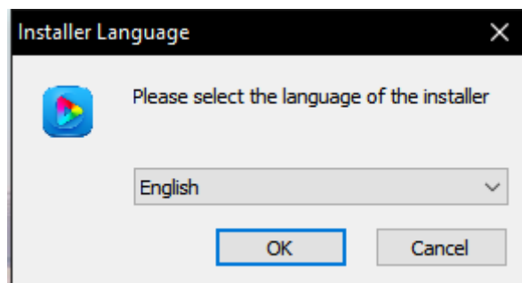
Figure 1-1 Installing language
