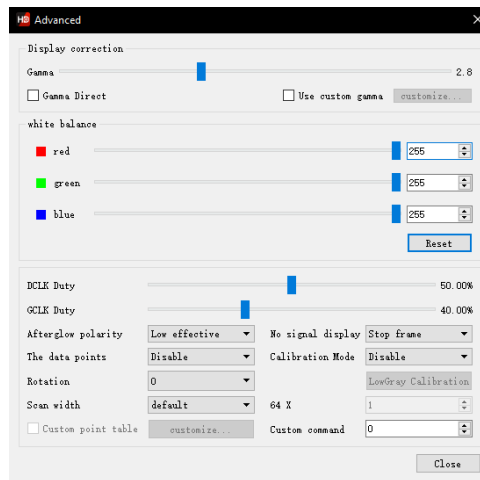
Figure 3-6 Advanced settings
